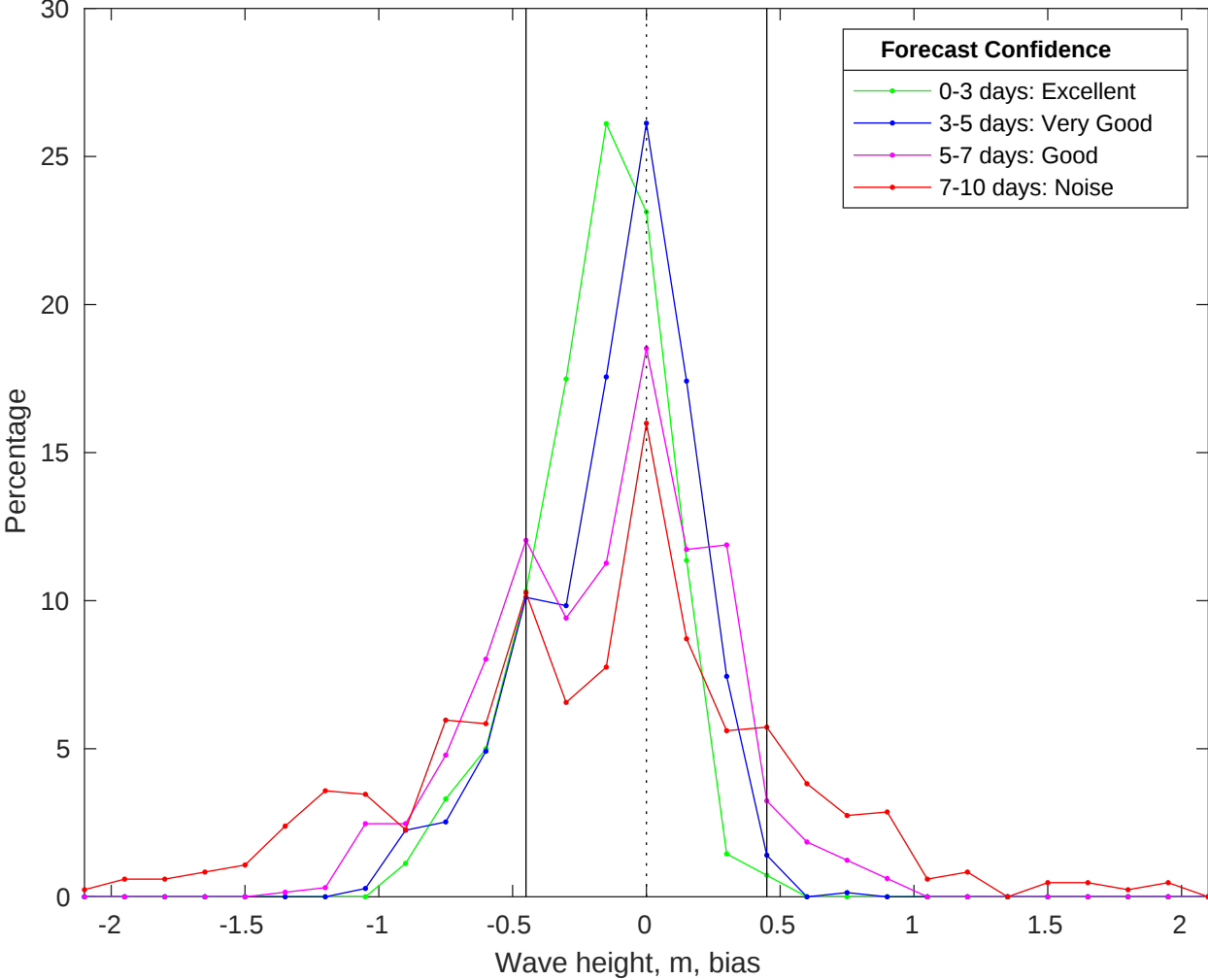
NDBC 46069 vs CMEMS Waves Bias Histogram: 21-Oct-2025
