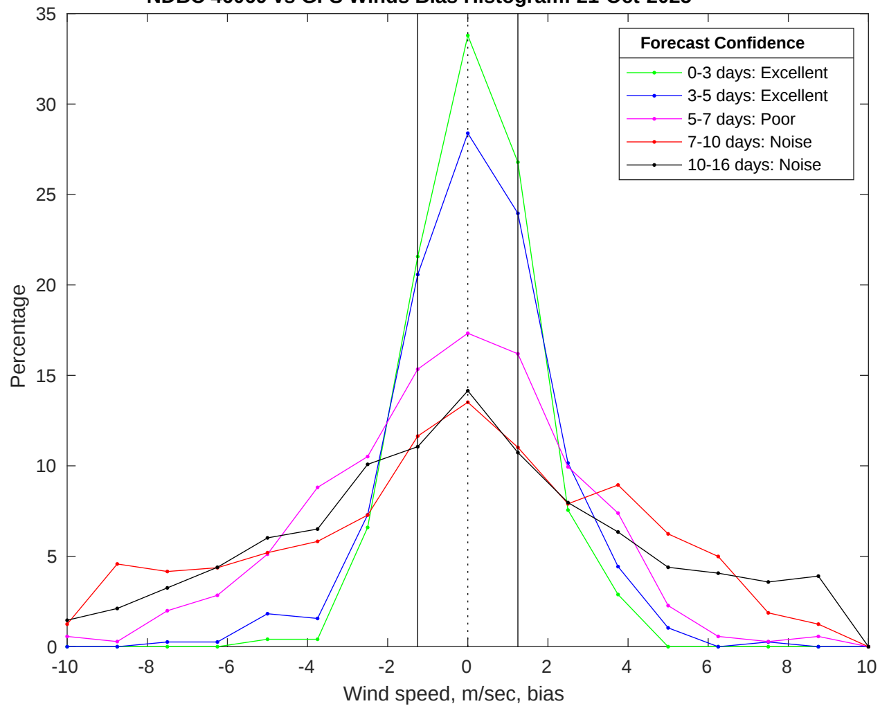
NDBC 46069 vs GFS Winds Bias Histogram: 21-Oct-2025
