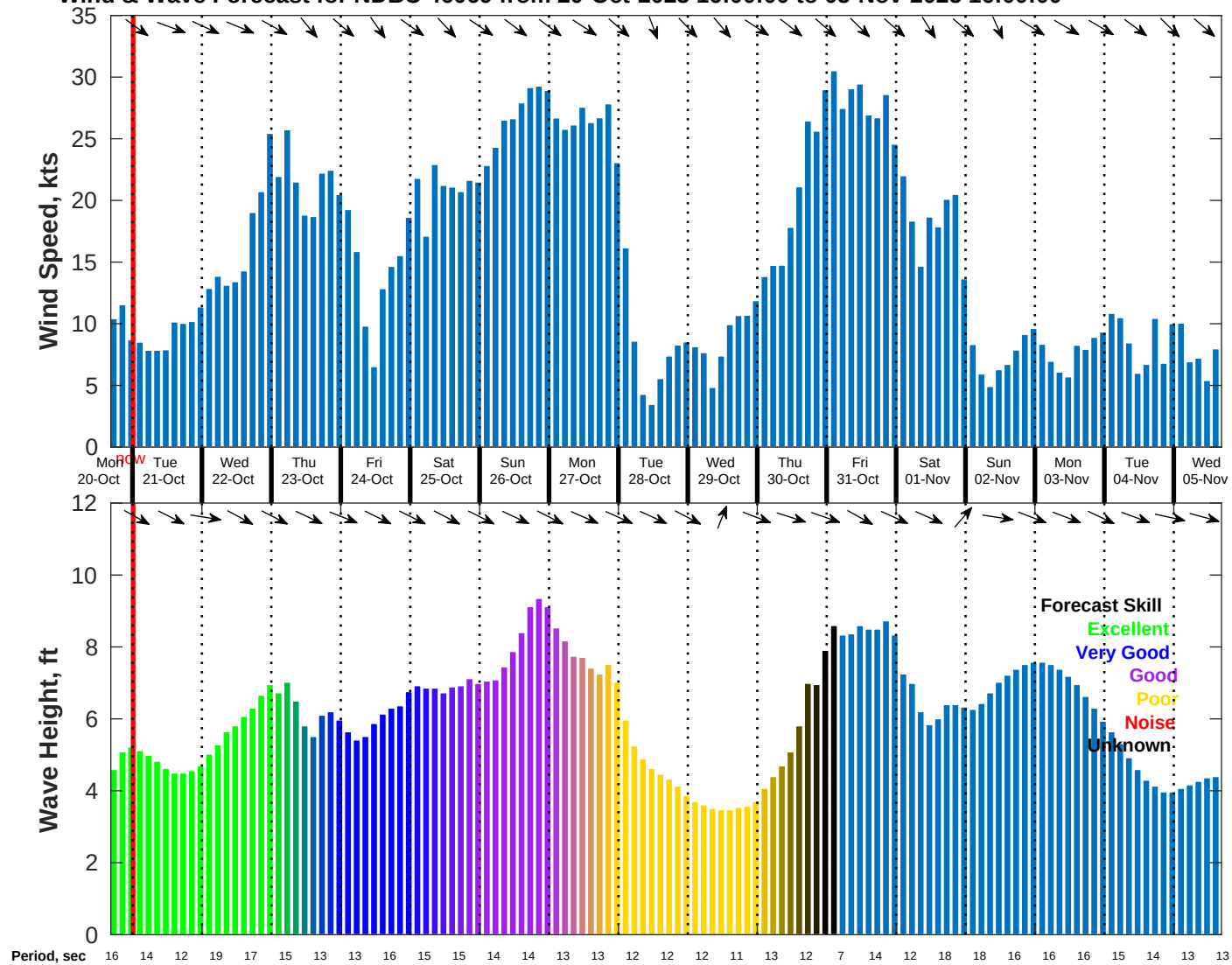
Wind & Wave Forecast for NDBC 46069 from 20-Oct-2025 16:00:00 to 05-Nov-2025 16:00:00
