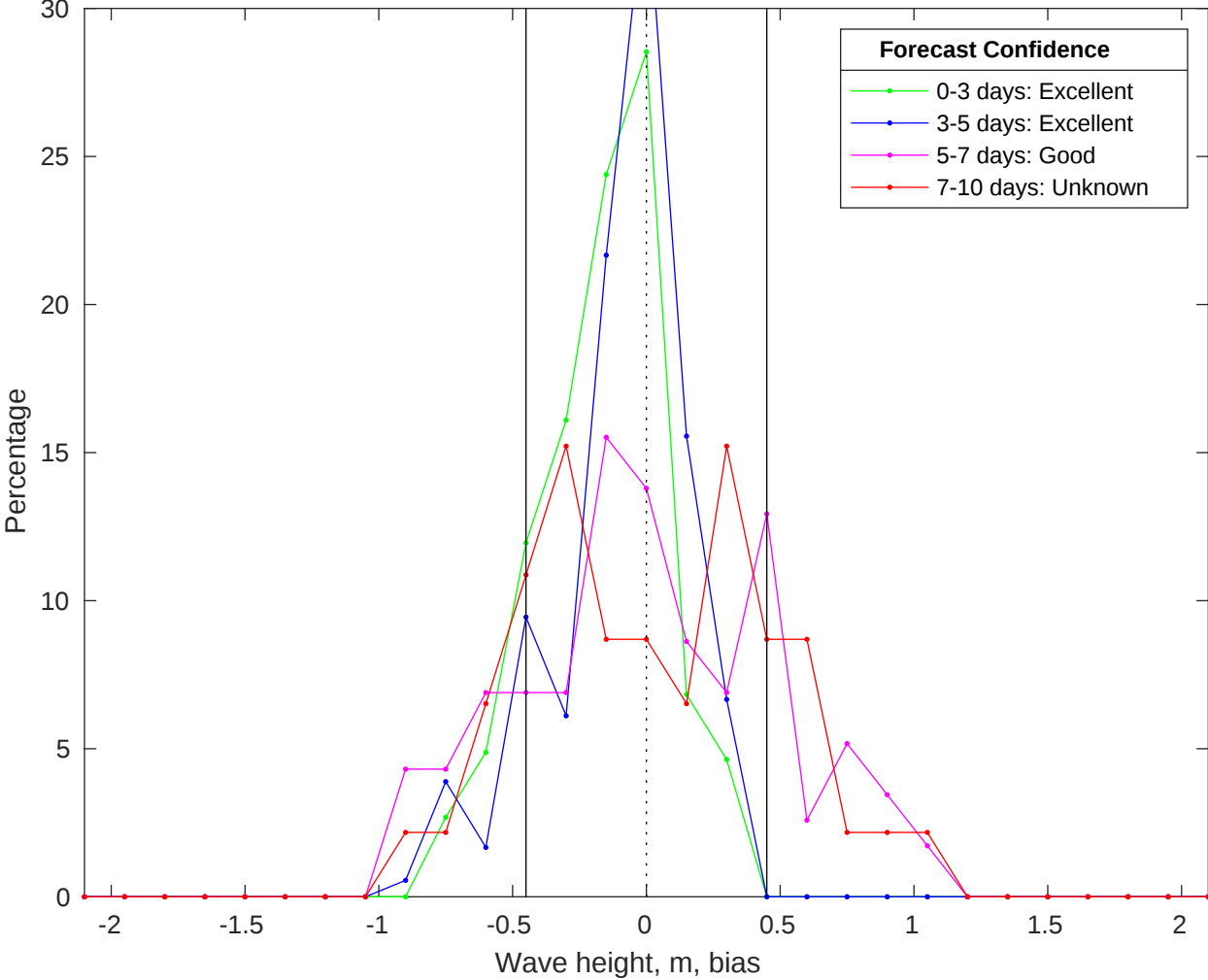
NDBC 46259 vs CMEMS Waves Bias Histogram: 21-Oct-2025
