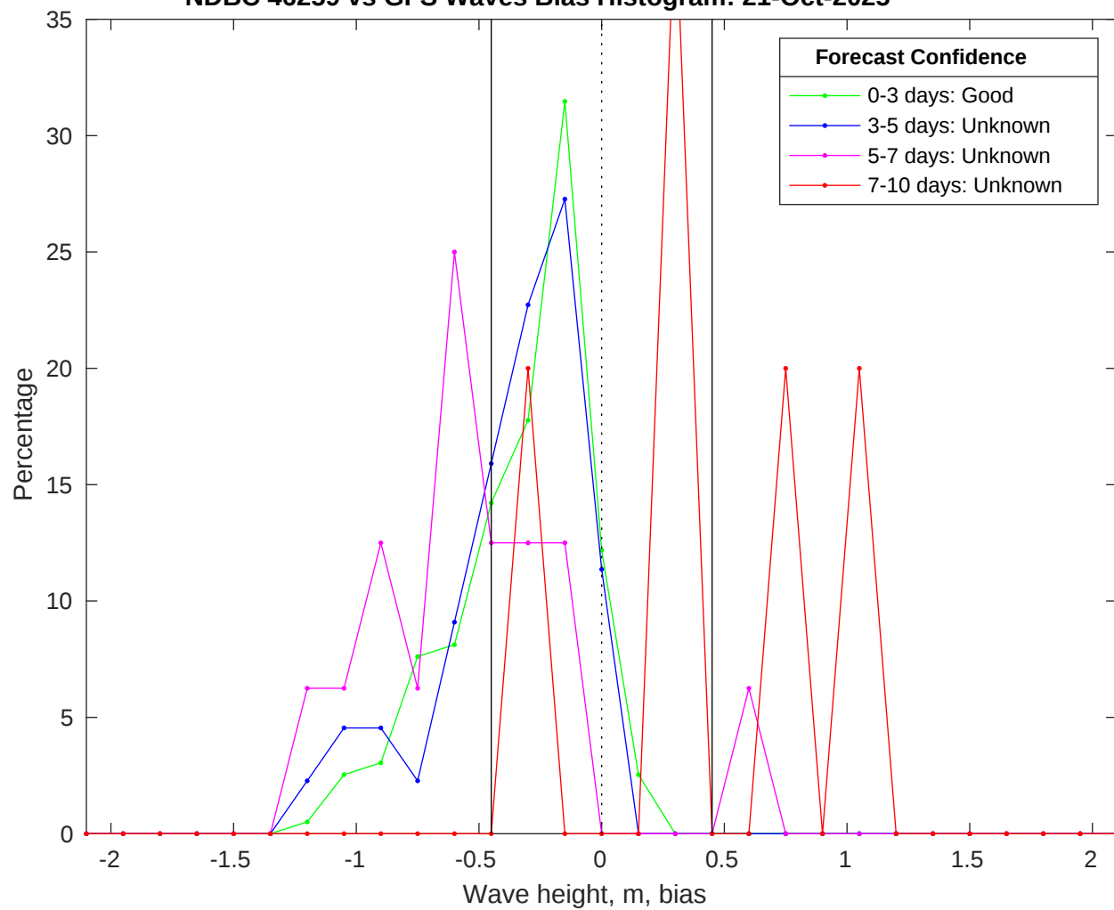
NDBC 46259 vs GFS Waves Bias Histogram: 21-Oct-2025
