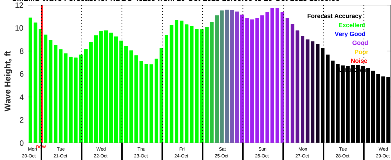
CMEMS Wave Forecast for NDBC 46259 from 20-Oct-2025 16:00:00 to 29-Oct-2025 16:00:00
