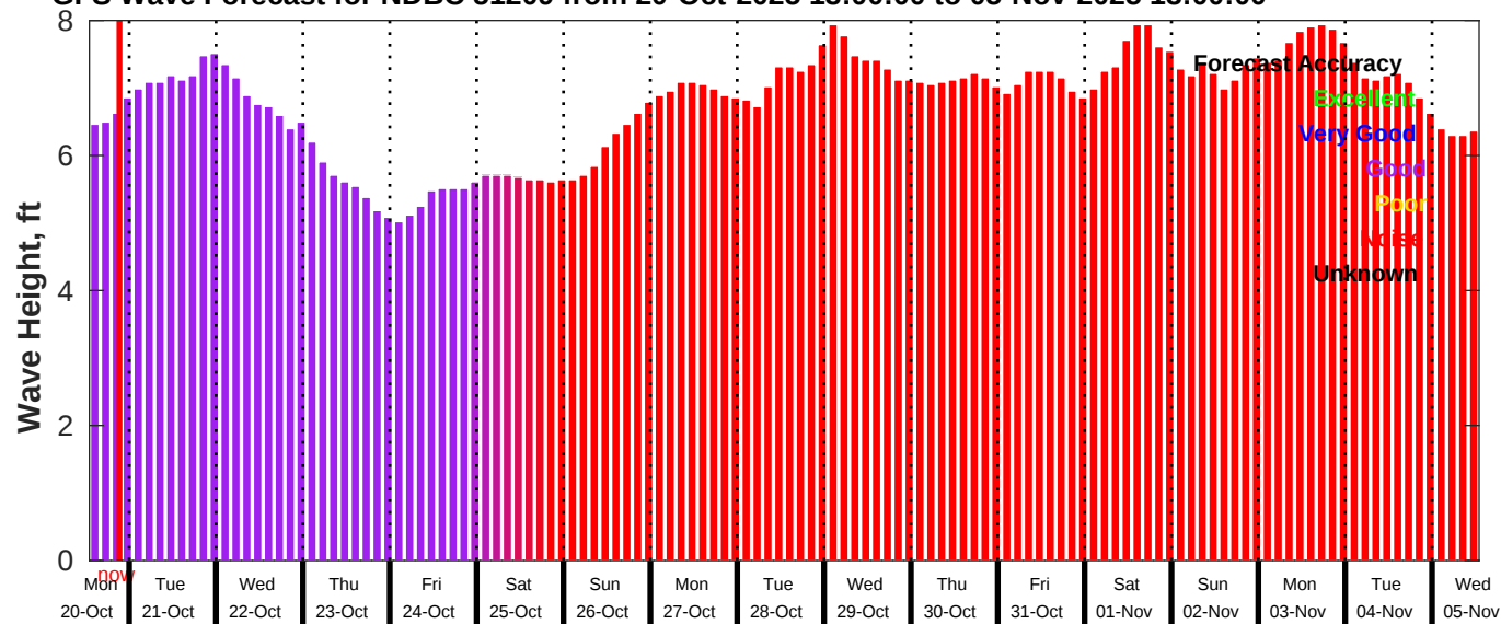
GFS Wave Forecast for NDBC 51209 from 20-Oct-2025 13:00:00 to 05-Nov-2025 13:00:00
