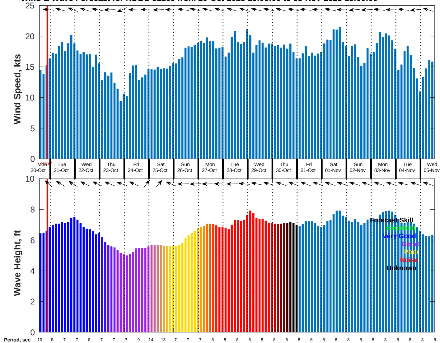
Wind & Wave Forecast for NDBC 51209 from 20-Oct-2025 13:00:00 to 05-Nov-2025 13:00:00
