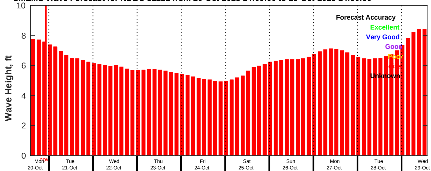
CMEMS Wave Forecast for NDBC 51211 from 20-Oct-2025 14:00:00 to 29-Oct-2025 14:00:00
