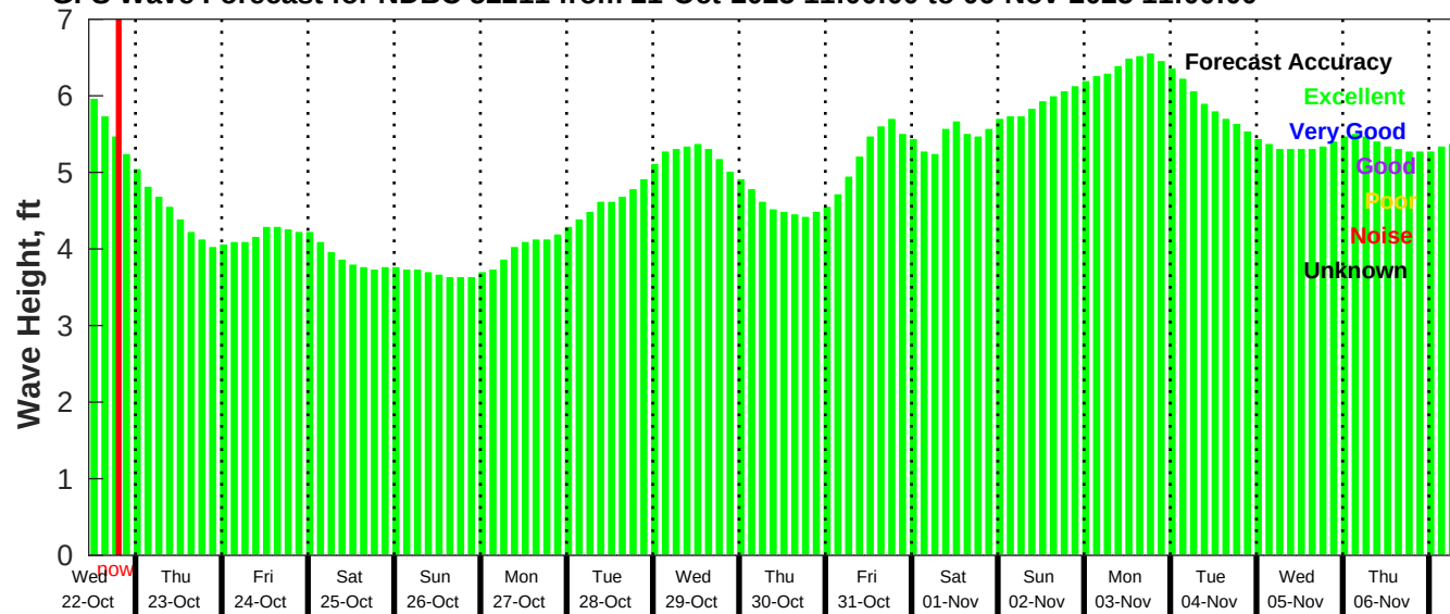
GFS Wave Forecast for NDBC 52211 from 21-Oct-2025 11:00:00 to 06-Nov-2025 11:00:00
