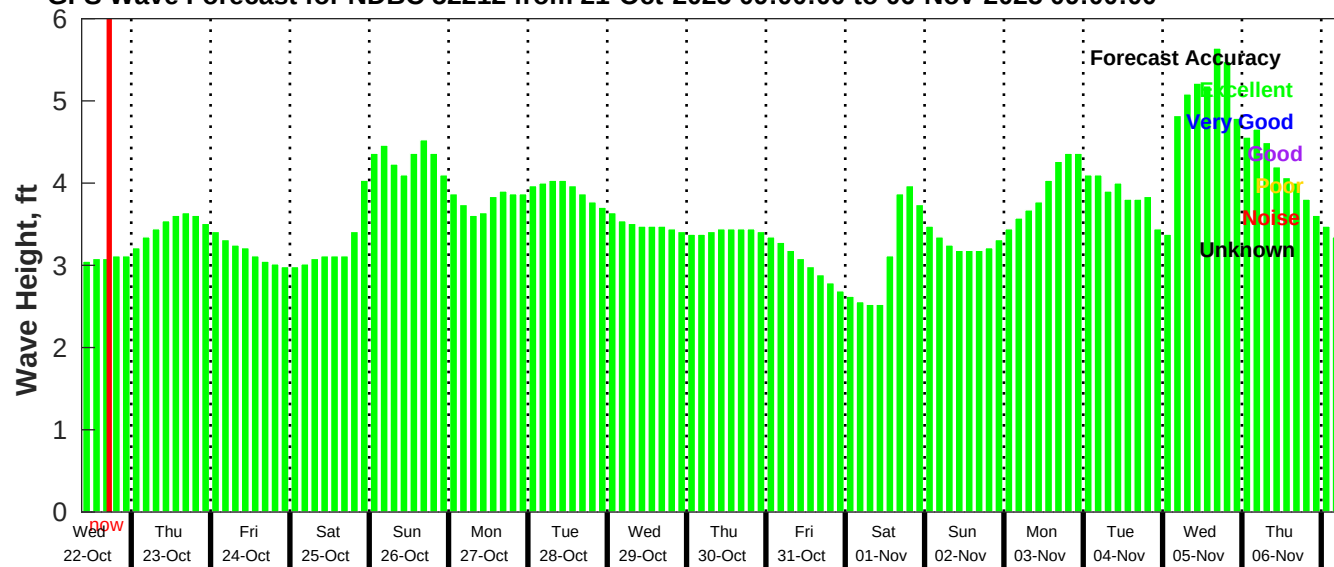
GFS Wave Forecast for NDBC 52212 from 21-Oct-2025 09:00:00 to 06-Nov-2025 09:00:00
