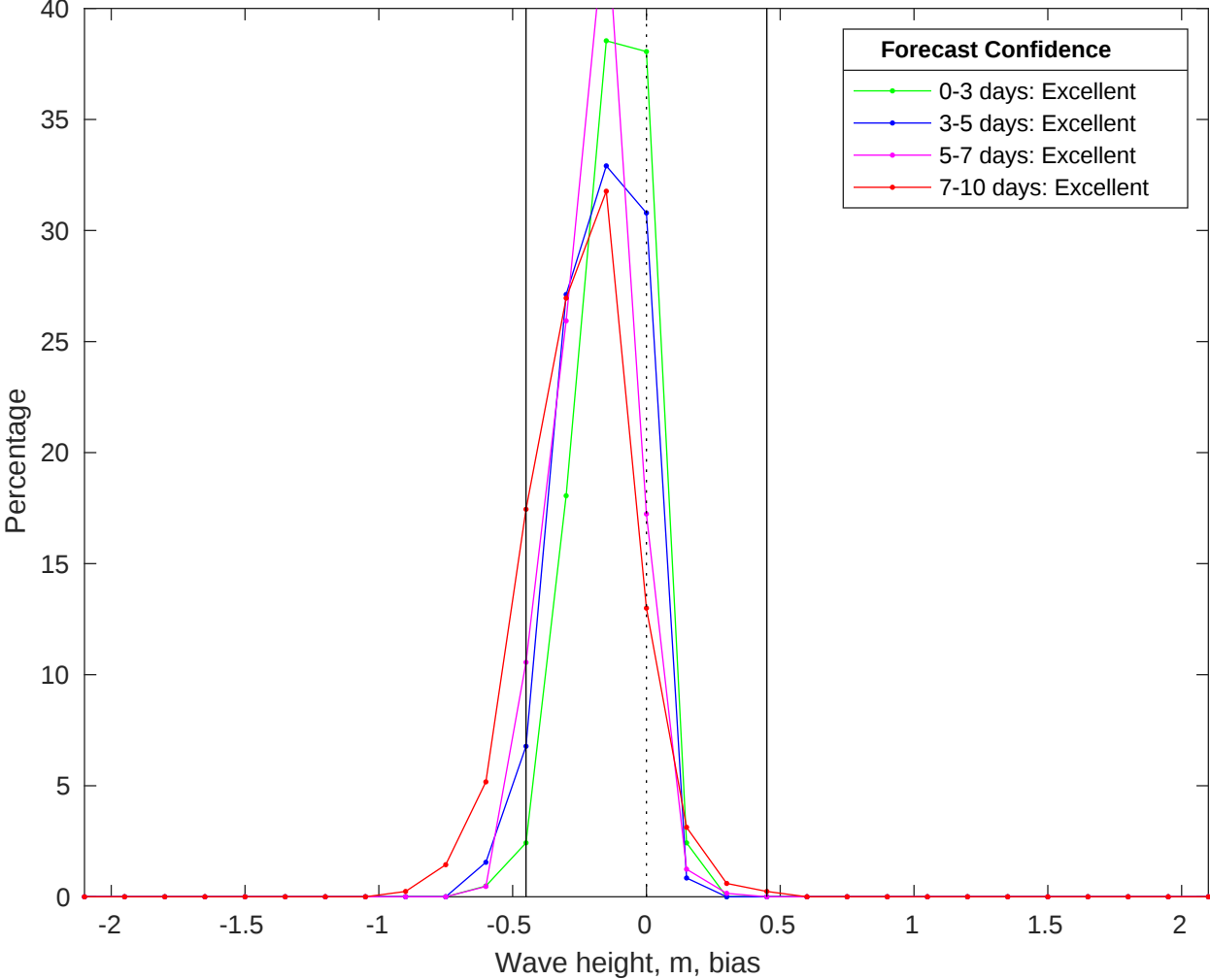
NDBC 52213 vs CMEMS Waves Bias Histogram: 21-Oct-2025
