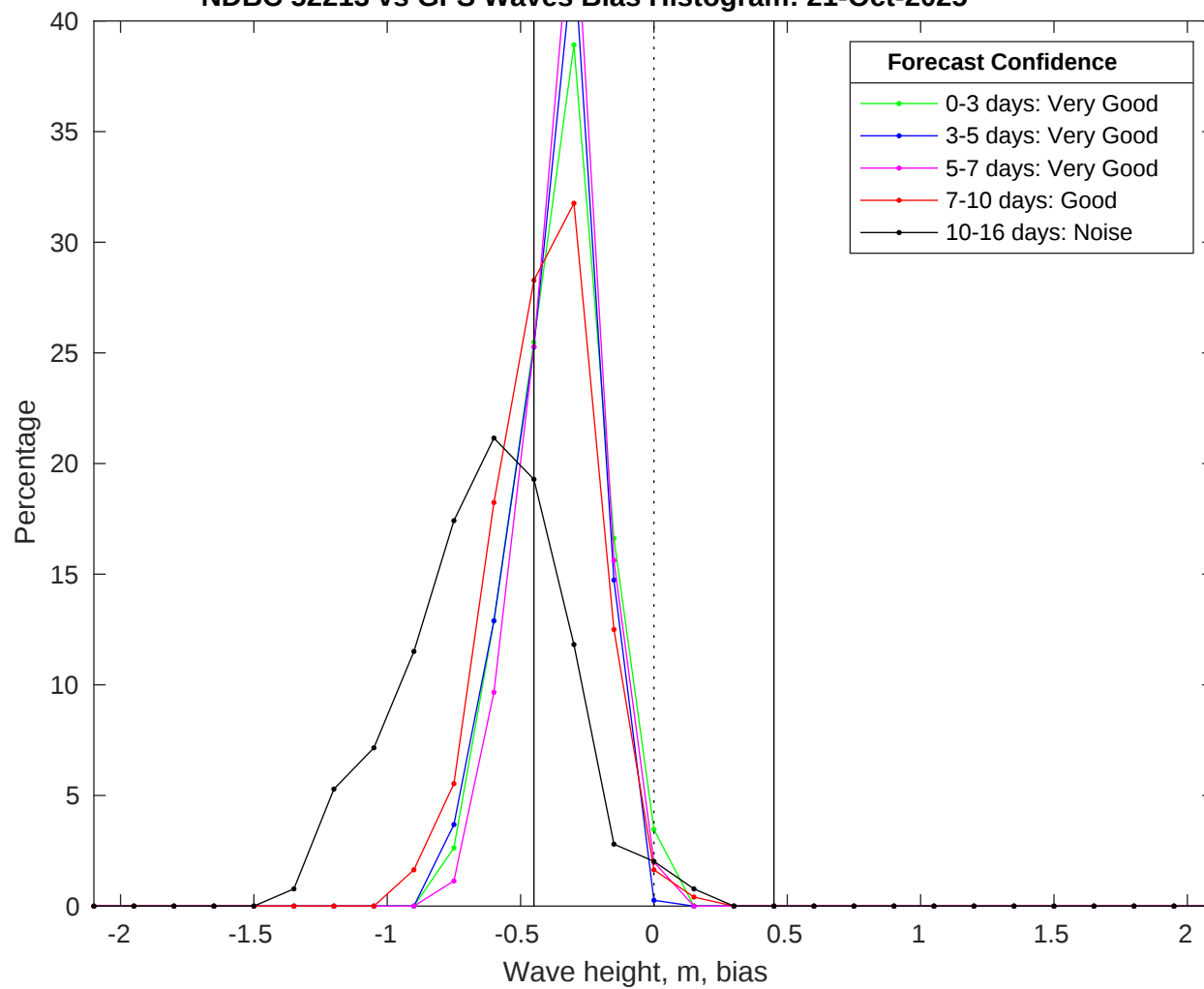
NDBC 52213 vs GFS Waves Bias Histogram: 21-Oct-2025
