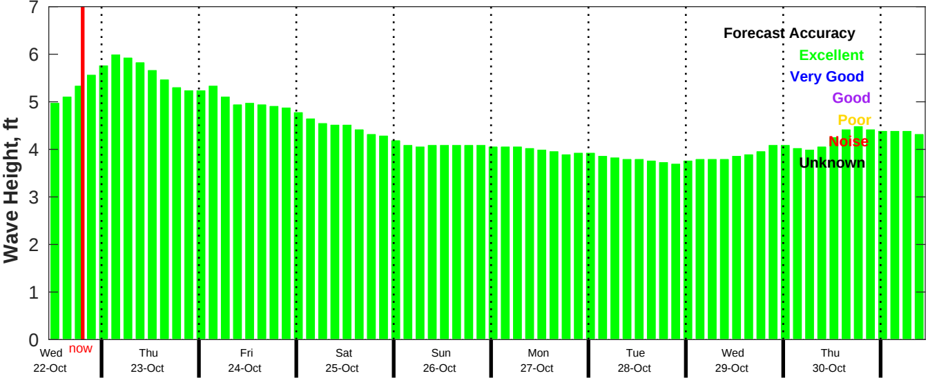
CMEMS Wave Forecast for NDBC 52213 from 21-Oct-2025 11:00:00 to 30-Oct-2025 11:00:00
