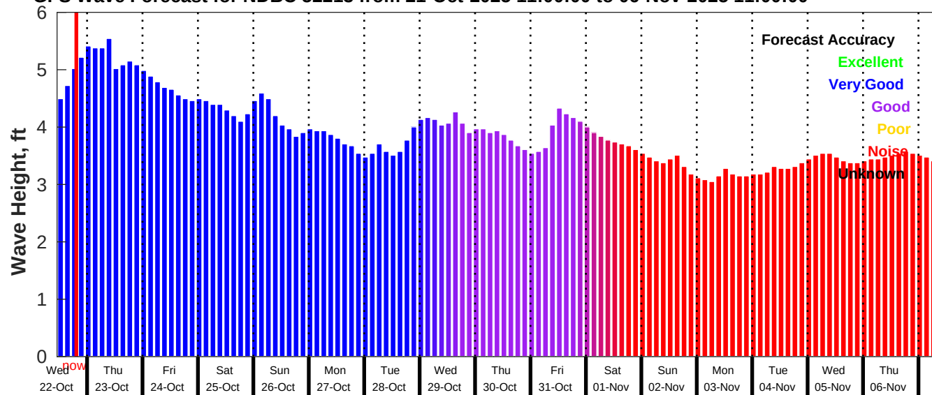
GFS Wave Forecast for NDBC 52213 from 21-Oct-2025 11:00:00 to 06-Nov-2025 11:00:00
