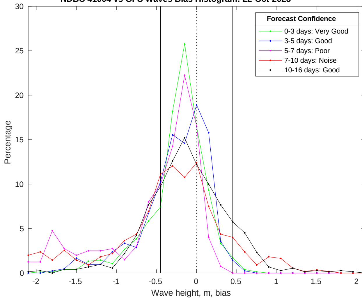
NDBC 41004 vs GFS Waves Bias Histogram: 22-Oct-2025
