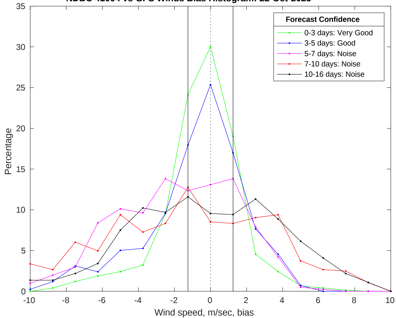
NDBC 41004 vs GFS Winds Bias Histogram: 22-Oct-2025
