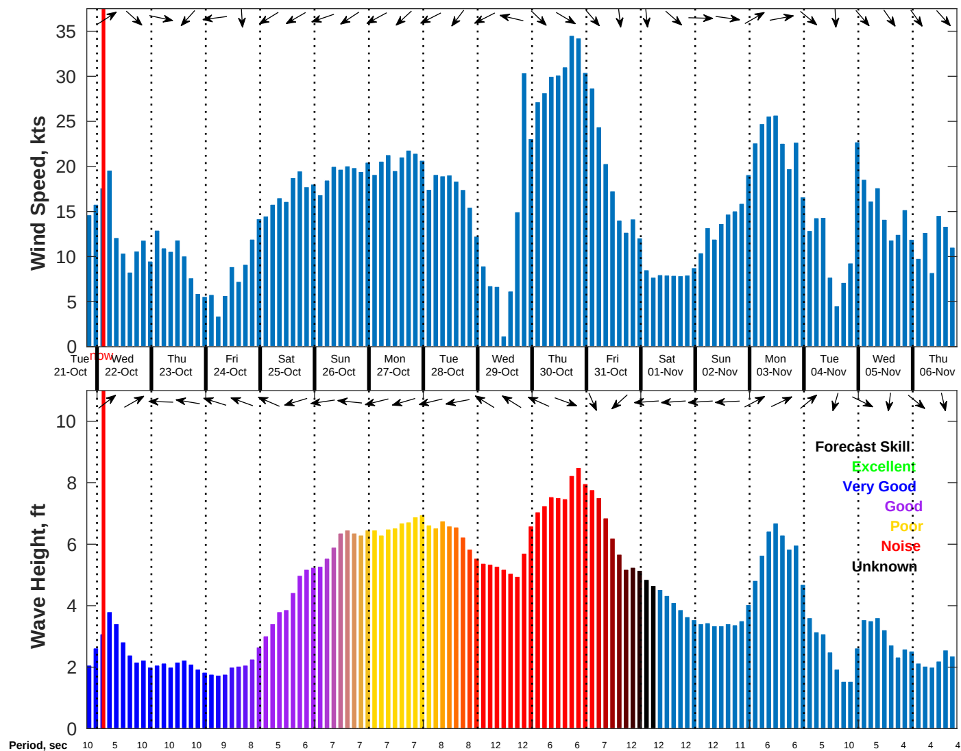
Wind & Wave Forecast for NDBC 41004 from 21-Oct-2025 19:00:00 to 06-Nov-2025 19:00:00
