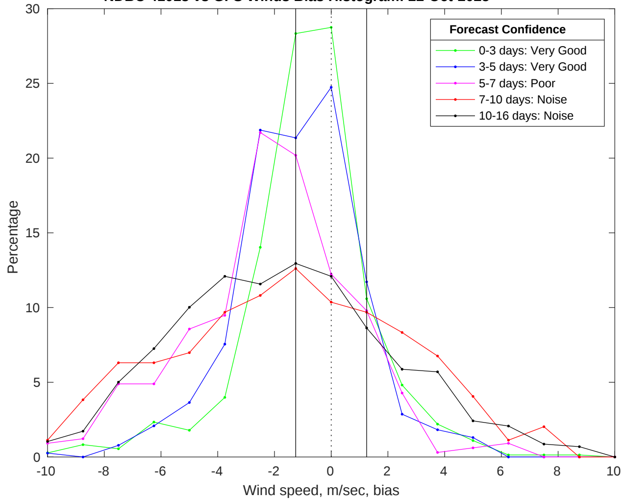
NDBC 41013 vs GFS Winds Bias Histogram: 22-Oct-2025
