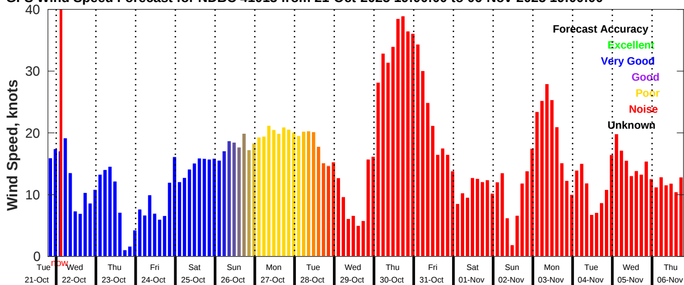
GFS Wind Speed Forecast for NDBC 41013 from 21-Oct-2025 19:00:00 to 06-Nov-2025 19:00:00
