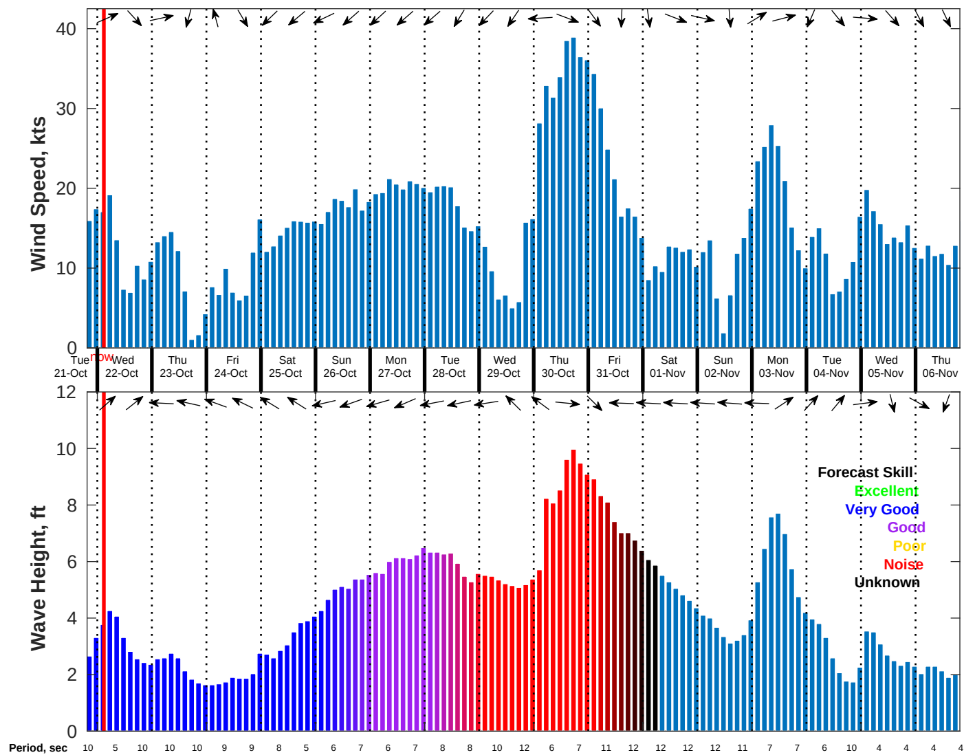
Wind & Wave Forecast for NDBC 41013 from 21-Oct-2025 19:00:00 to 06-Nov-2025 19:00:00
