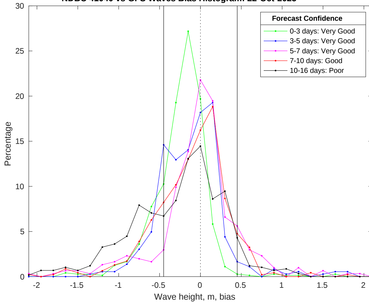
NDBC 41040 vs GFS Waves Bias Histogram: 22-Oct-2025
