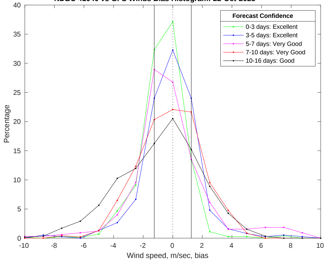
NDBC 41040 vs GFS Winds Bias Histogram: 22-Oct-2025
