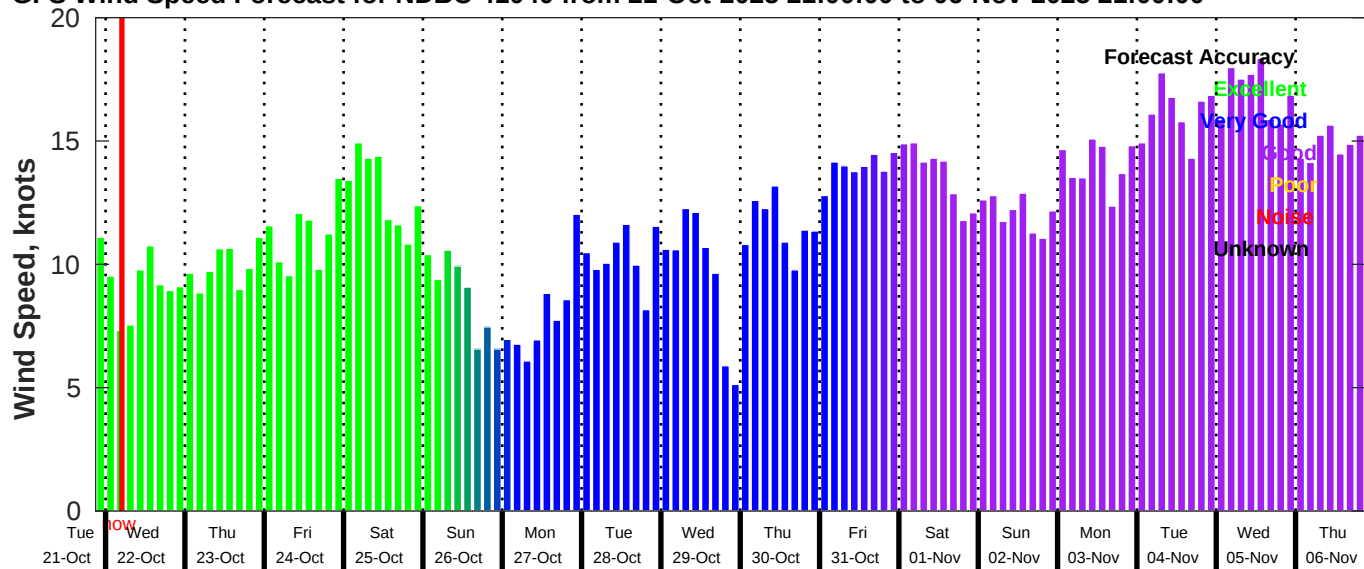
GFS Wind Speed Forecast for NDBC 41040 from 21-Oct-2025 21:00:00 to 06-Nov-2025 21:00:00
