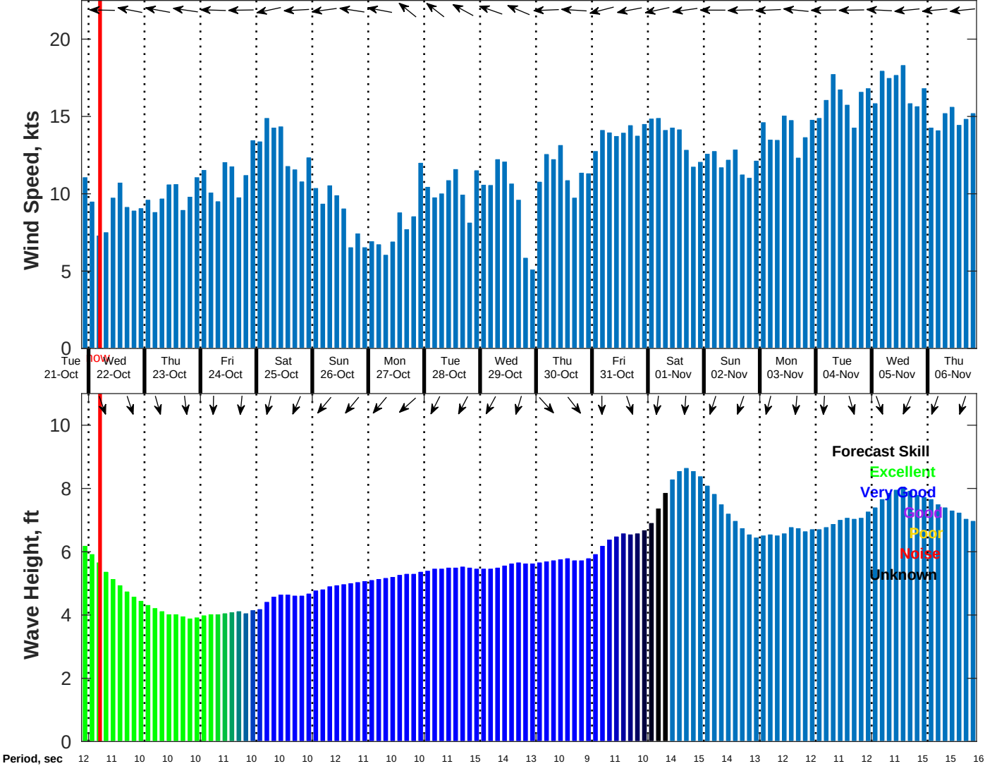
Wind & Wave Forecast for NDBC 41040 from 21-Oct-2025 21:00:00 to 06-Nov-2025 21:00:00
