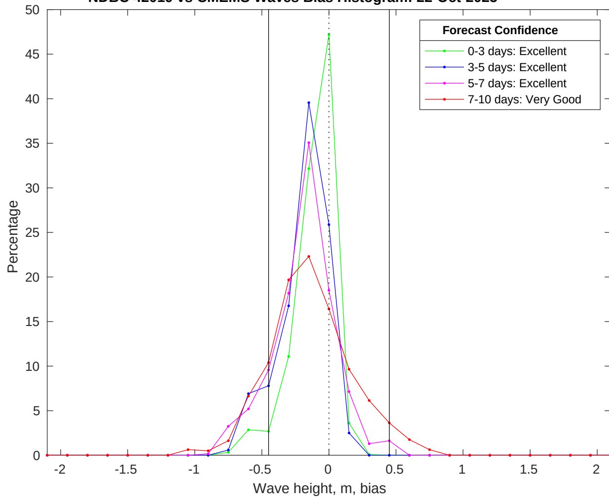
NDBC 42019 vs CMEMS Waves Bias Histogram: 22-Oct-2025
