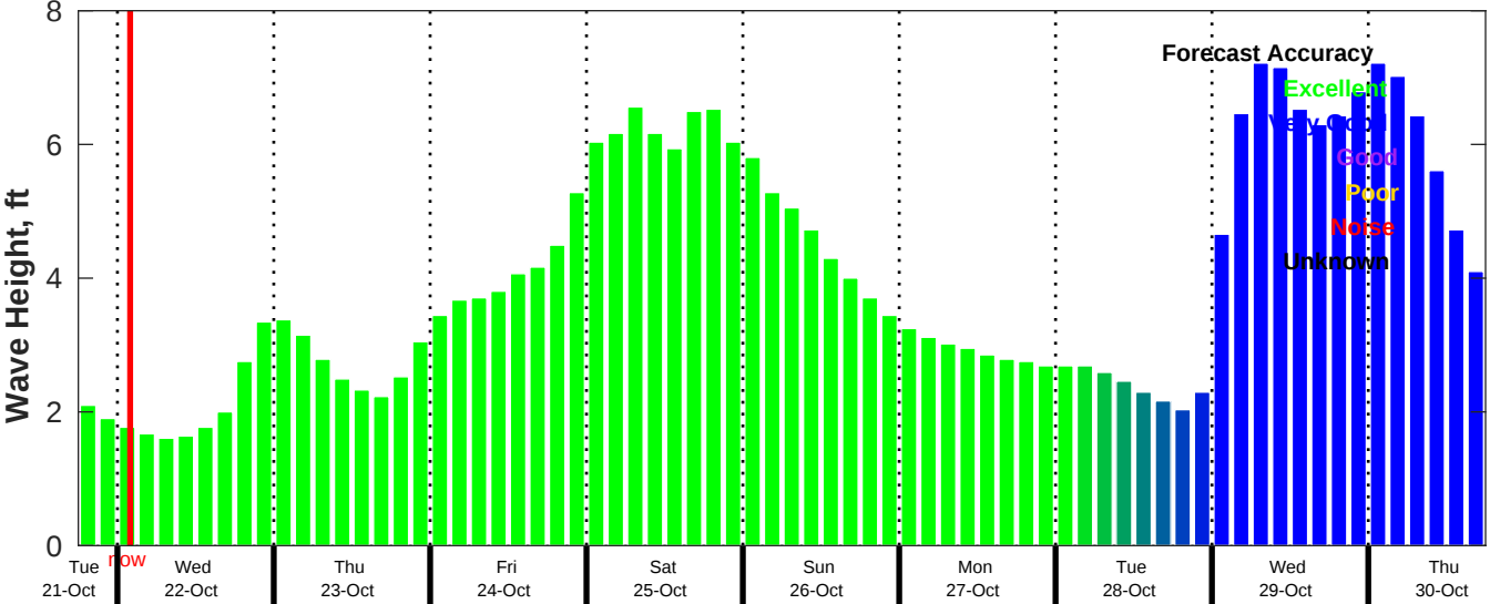
CMEMS Wave Forecast for NDBC 42019 from 21-Oct-2025 18:00:00 to 30-Oct-2025 18:00:00
