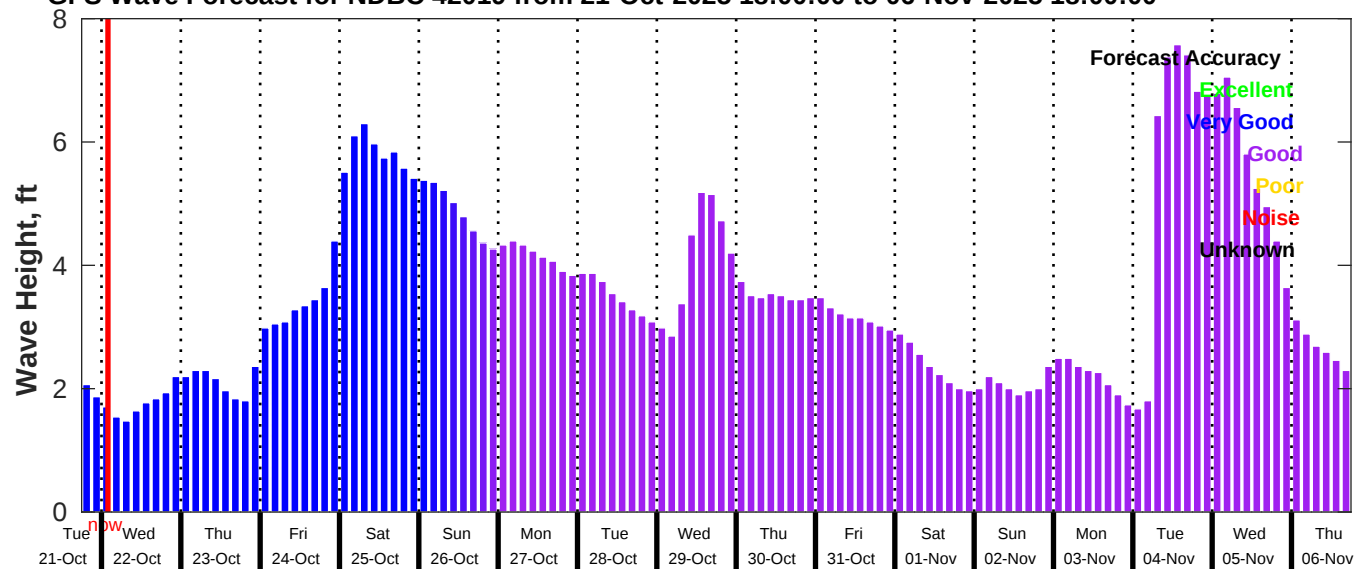
GFS Wave Forecast for NDBC 42019 from 21-Oct-2025 18:00:00 to 06-Nov-2025 18:00:00
