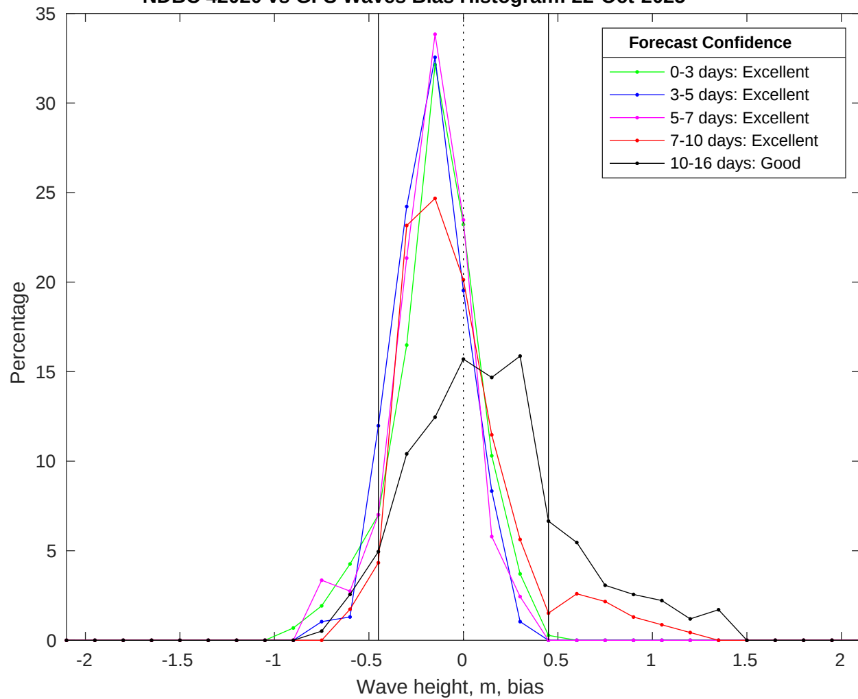
NDBC 42020 vs GFS Waves Bias Histogram: 22-Oct-2025
