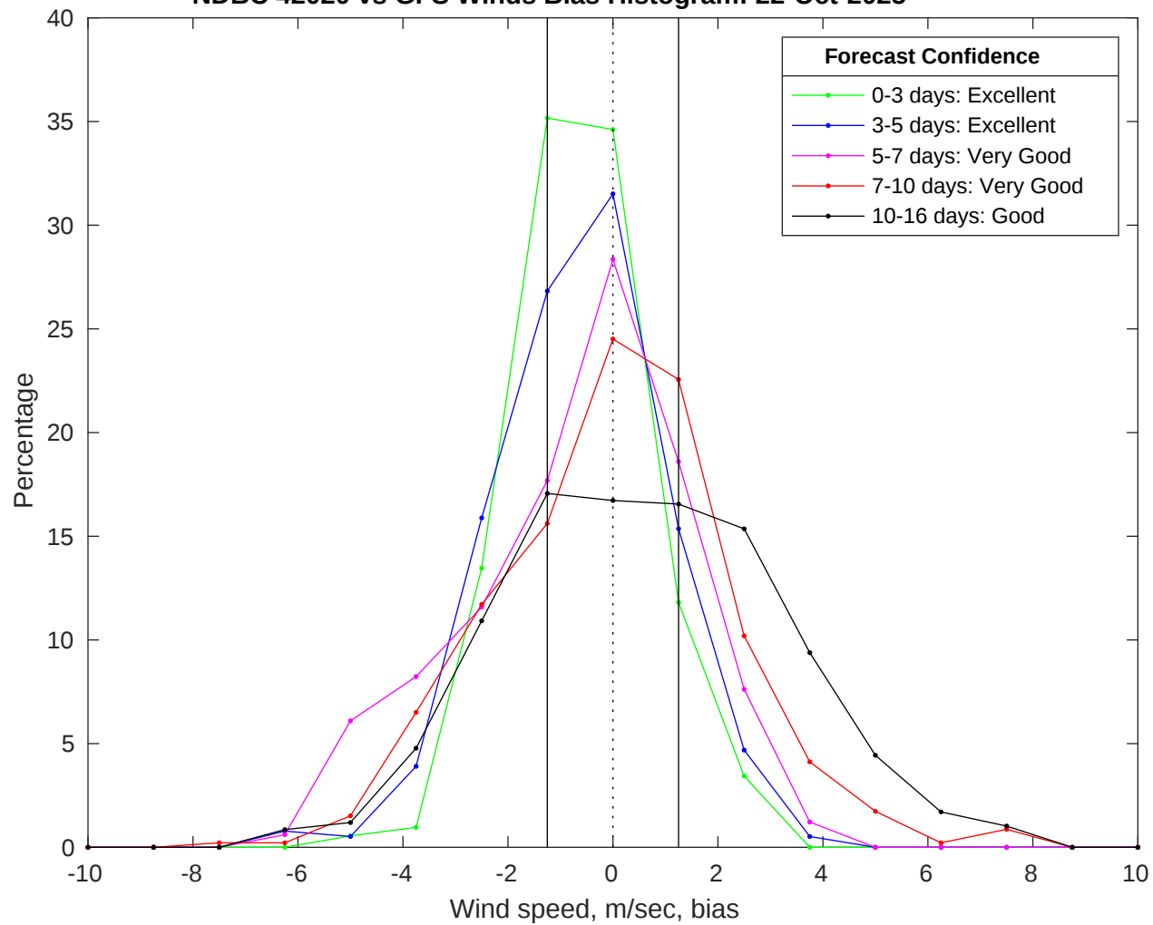
NDBC 42020 vs GFS Winds Bias Histogram: 22-Oct-2025
