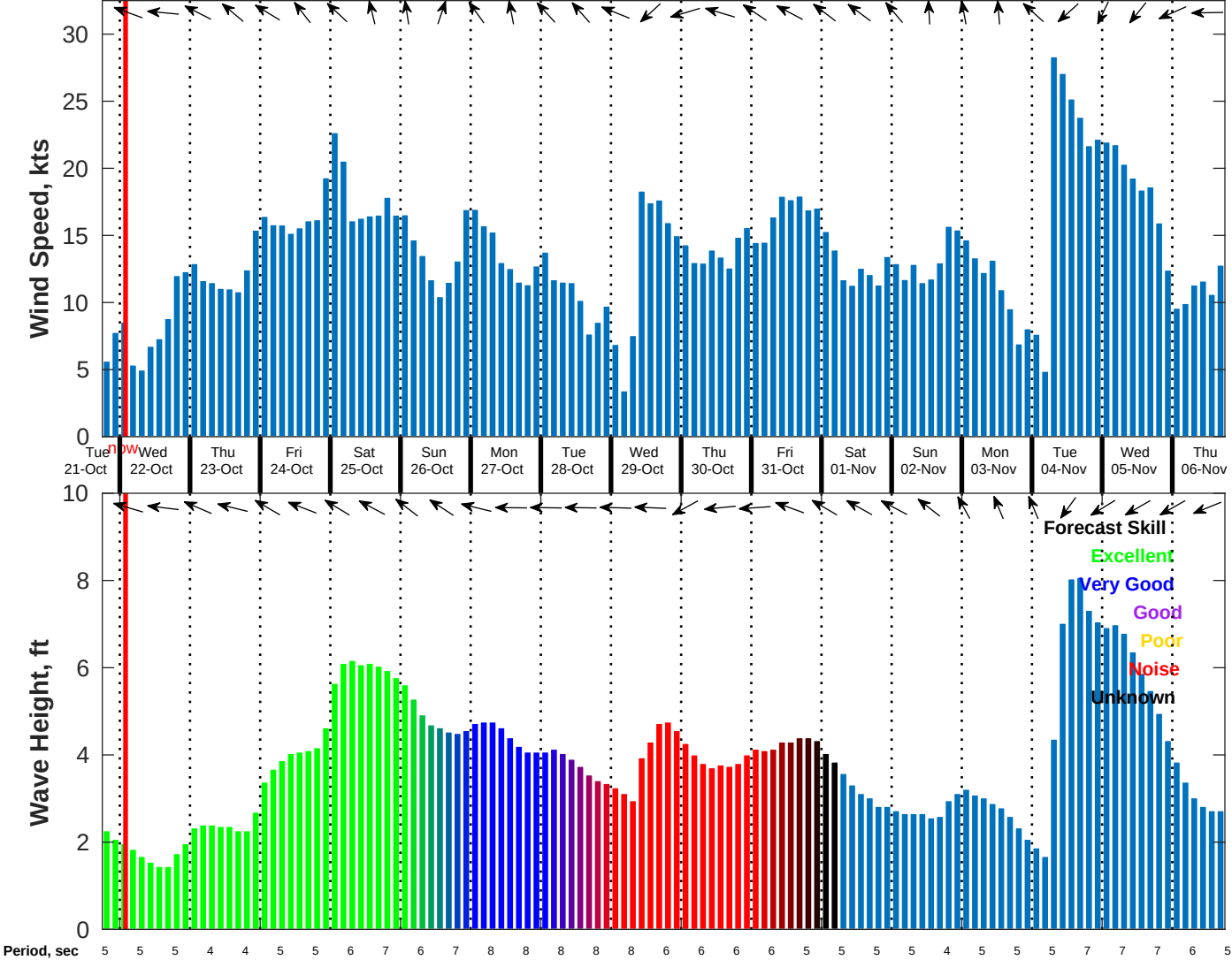
Wind & Wave Forecast for NDBC 42020 from 21-Oct-2025 18:00:00 to 06-Nov-2025 18:00:00
