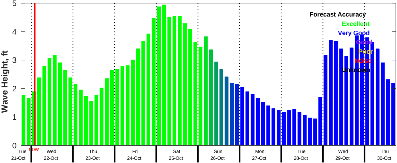
CMEMS Wave Forecast for NDBC 42035 from 21-Oct-2025 18:00:00 to 30-Oct-2025 18:00:00
