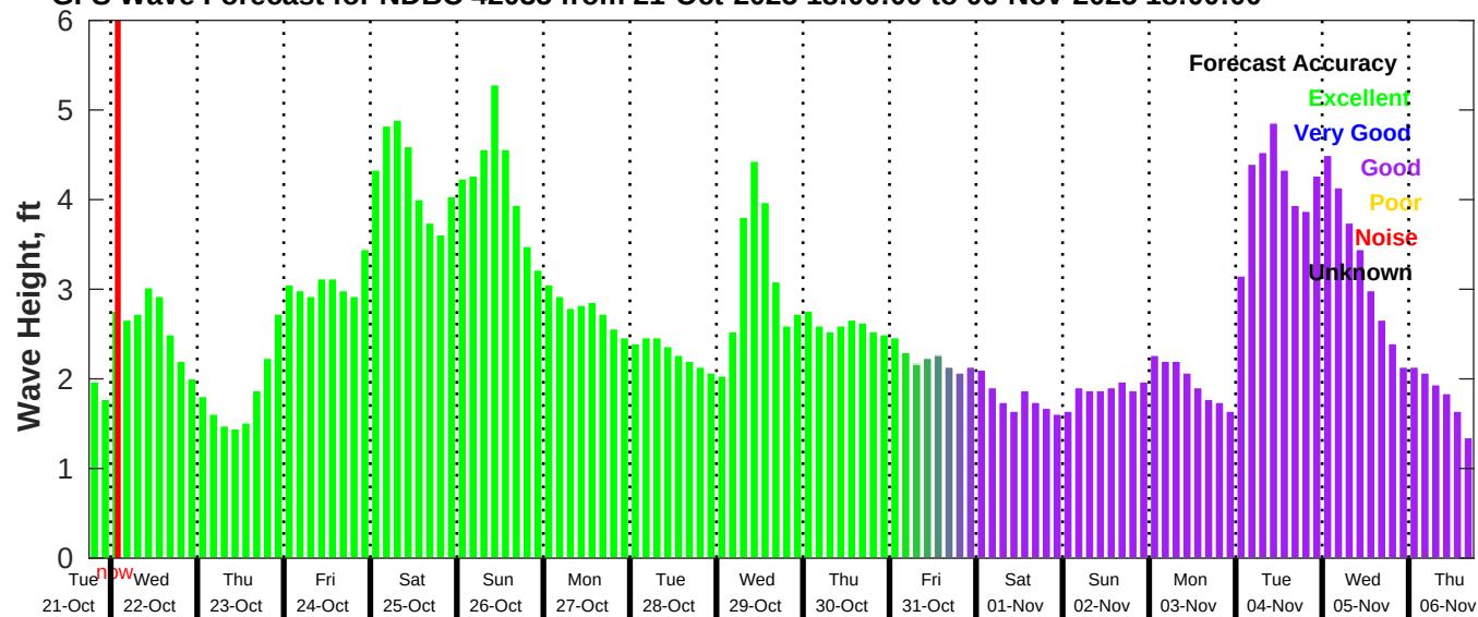
GFS Wave Forecast for NDBC 42035 from 21-Oct-2025 18:00:00 to 06-Nov-2025 18:00:00
