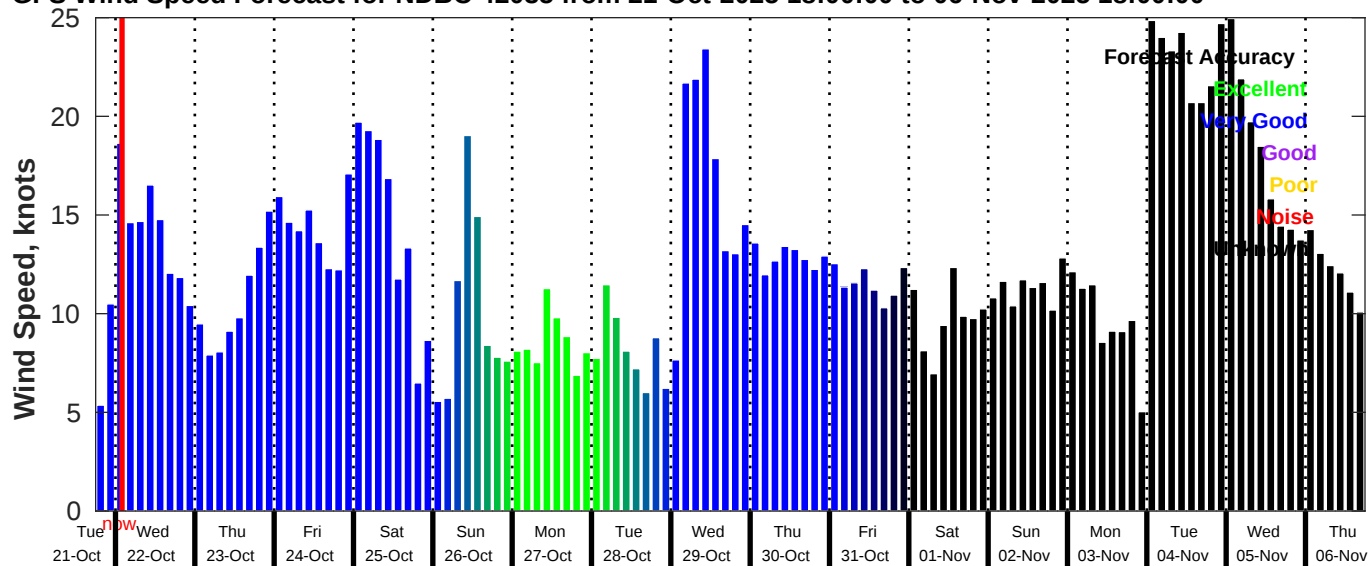
GFS Wind Speed Forecast for NDBC 42035 from 21-Oct-2025 18:00:00 to 06-Nov-2025 18:00:00
