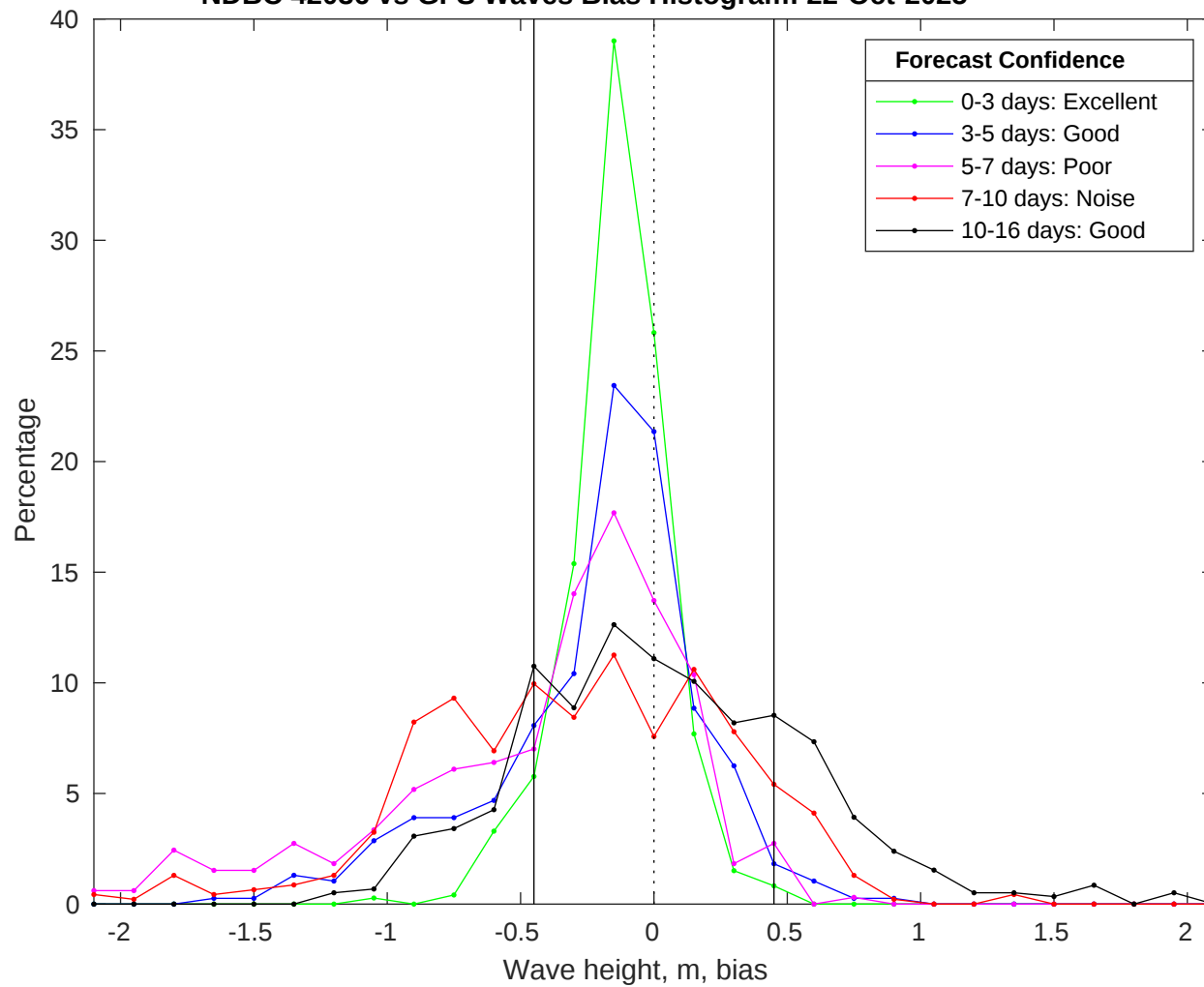
NDBC 42036 vs GFS Waves Bias Histogram: 22-Oct-2025
