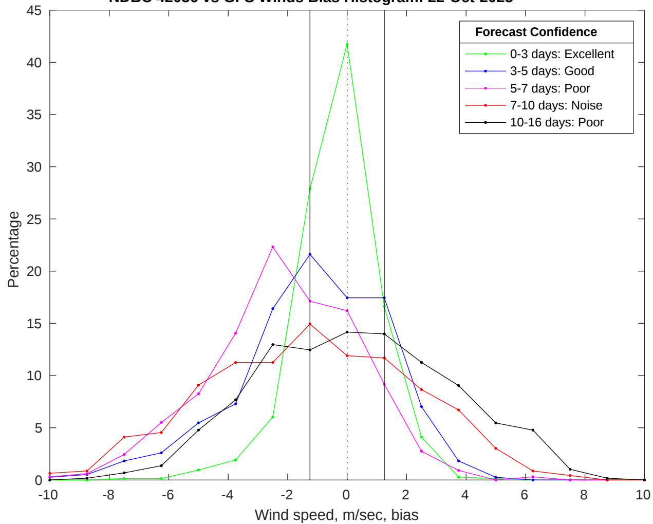
NDBC 42036 vs GFS Winds Bias Histogram: 22-Oct-2025
