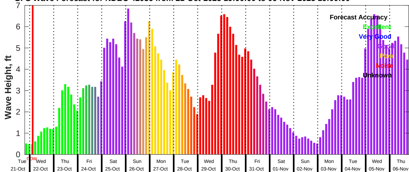
GFS Wave Forecast for NDBC 42036 from 21-Oct-2025 19:00:00 to 06-Nov-2025 19:00:00
