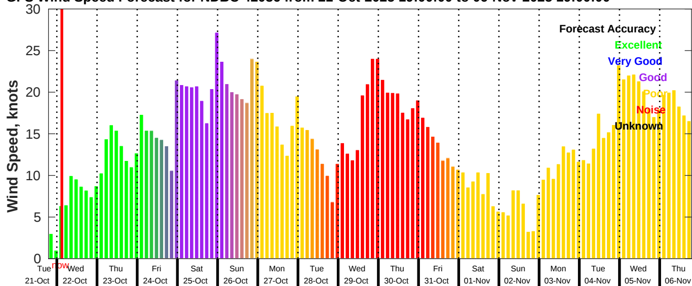
GFS Wind Speed Forecast for NDBC 42036 from 21-Oct-2025 19:00:00 to 06-Nov-2025 19:00:00
