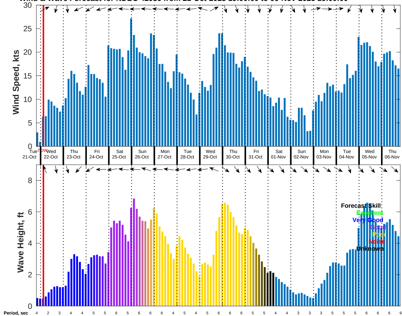
Wind & Wave Forecast for NDBC 42036 from 21-Oct-2025 19:00:00 to 06-Nov-2025 19:00:00
