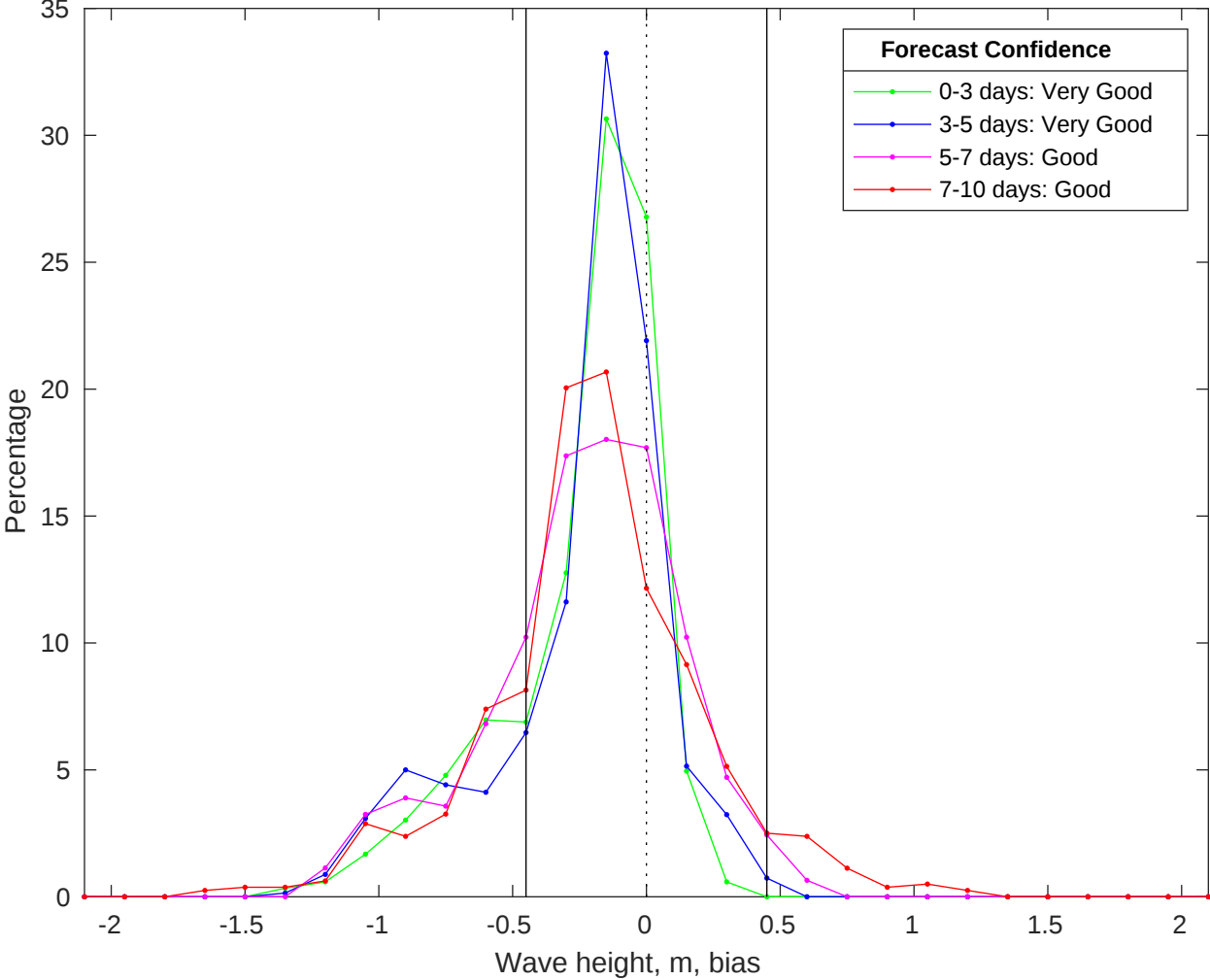
NDBC 42040 vs CMEMS Waves Bias Histogram: 22-Oct-2025
