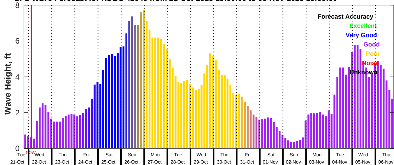
GFS Wave Forecast for NDBC 42040 from 21-Oct-2025 19:00:00 to 06-Nov-2025 19:00:00
