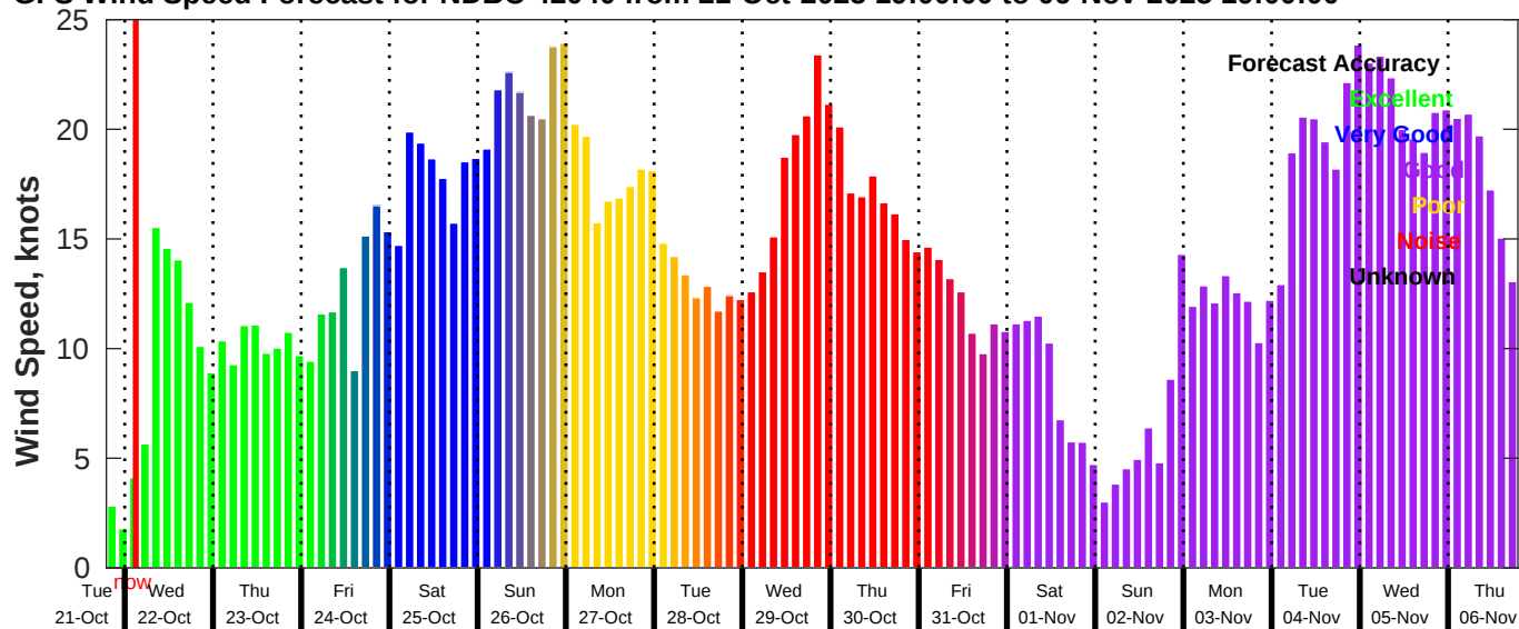
GFS Wind Speed Forecast for NDBC 42040 from 21-Oct-2025 19:00:00 to 06-Nov-2025 19:00:00
