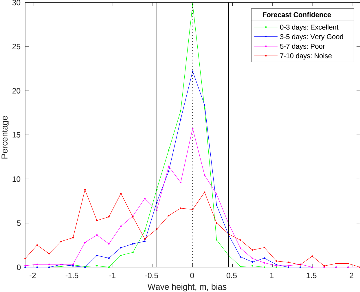
NDBC 44008 vs CMEMS Waves Bias Histogram: 22-Oct-2025
