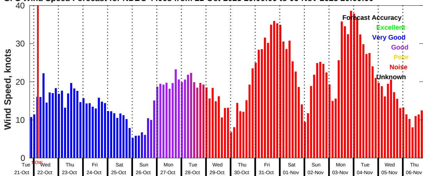
GFS Wind Speed Forecast for NDBC 44008 from 21-Oct-2025 20:00:00 to 06-Nov-2025 20:00:00
