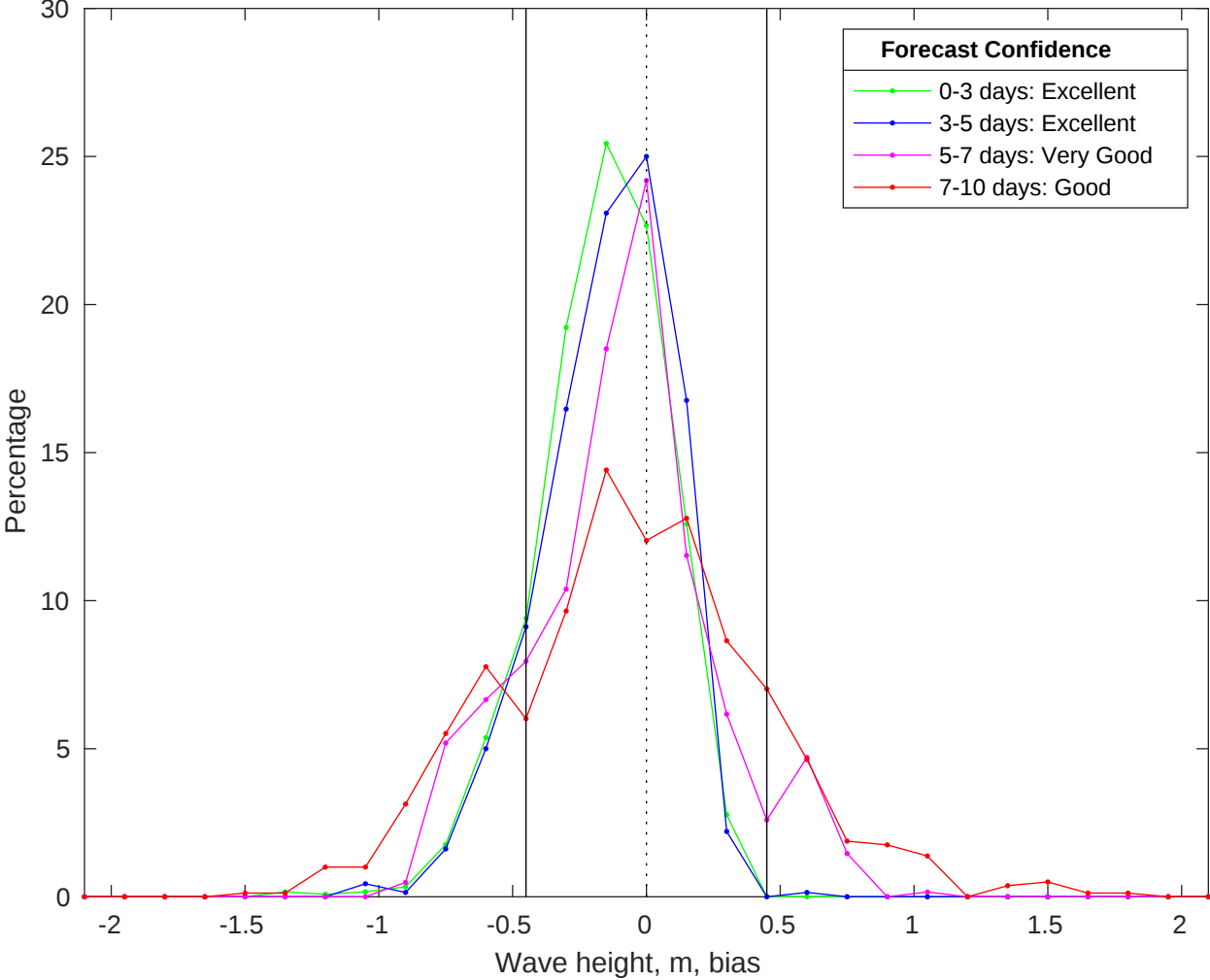
NDBC 46011 vs CMEMS Waves Bias Histogram: 22-Oct-2025
