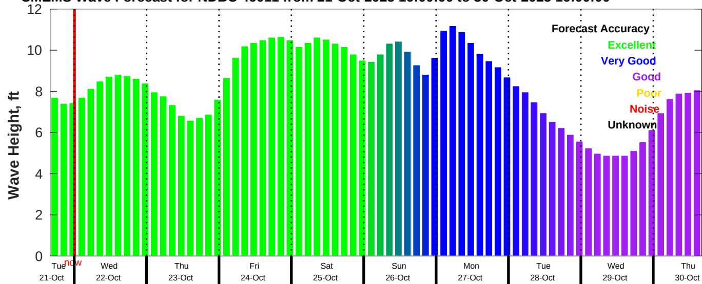
CMEMS Wave Forecast for NDBC 46011 from 21-Oct-2025 16:00:00 to 30-Oct-2025 16:00:00
