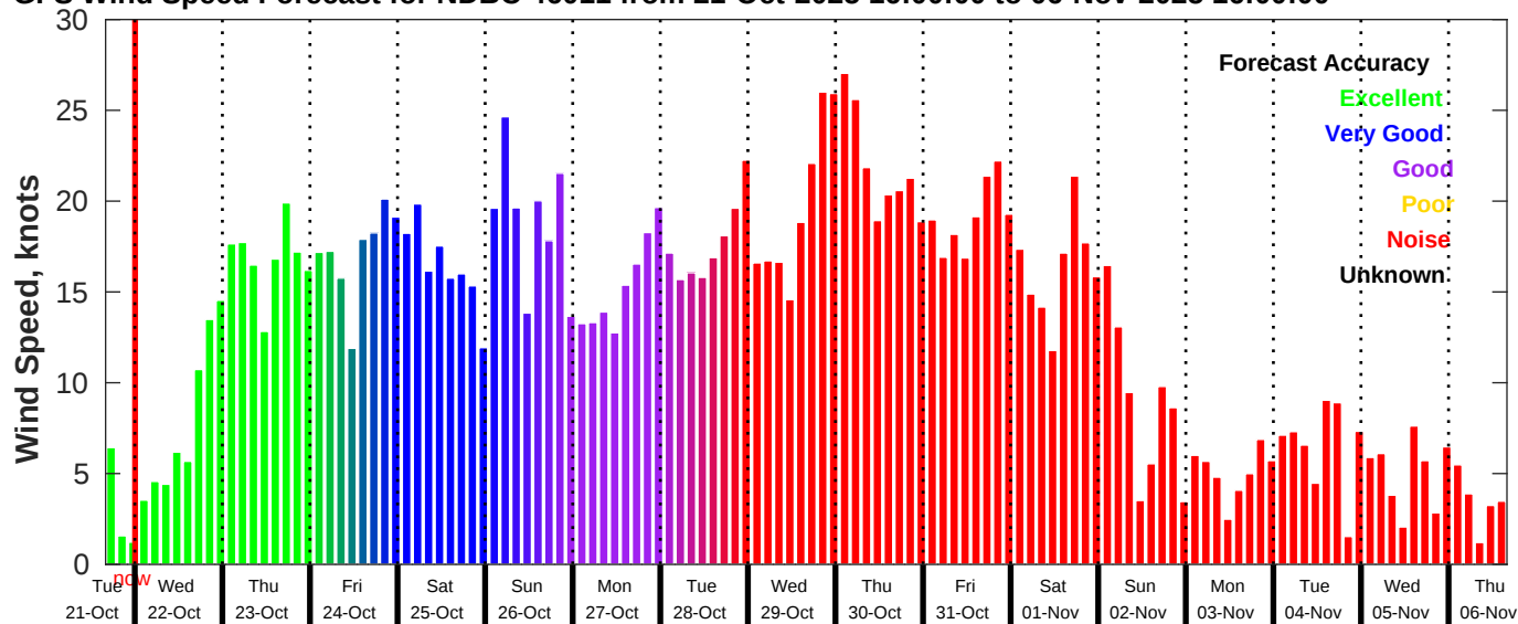
GFS Wind Speed Forecast for NDBC 46011 from 21-Oct-2025 16:00:00 to 06-Nov-2025 16:00:00
