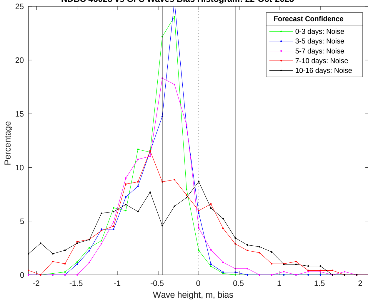
NDBC 46028 vs GFS Waves Bias Histogram: 22-Oct-2025
