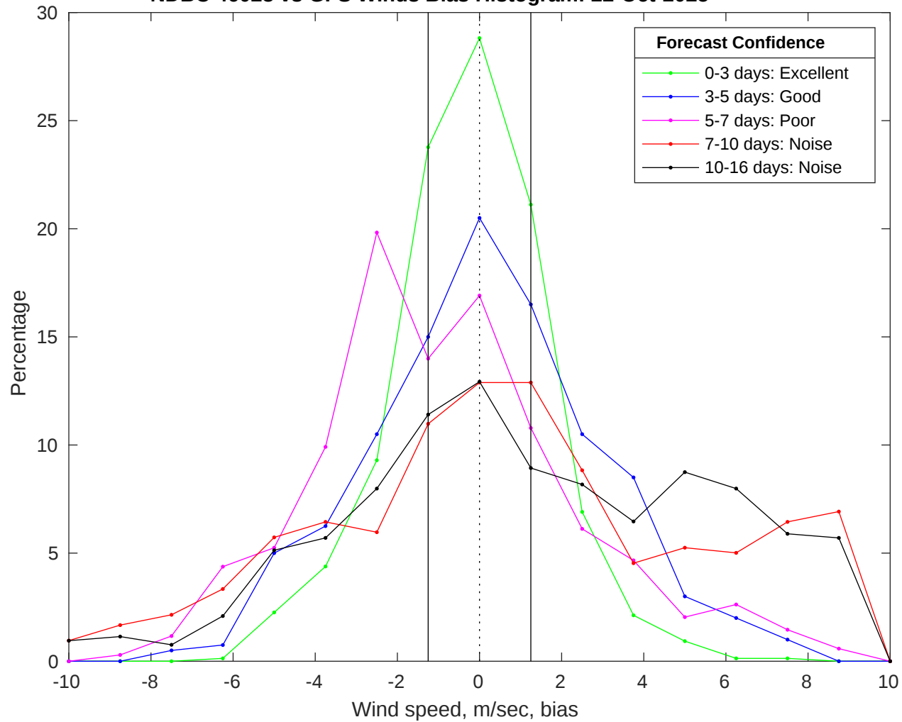
NDBC 46028 vs GFS Winds Bias Histogram: 22-Oct-2025
