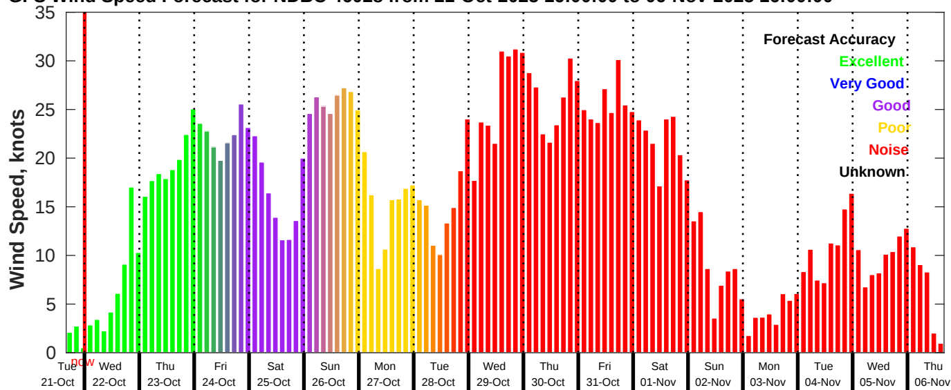
GFS Wind Speed Forecast for NDBC 46028 from 21-Oct-2025 16:00:00 to 06-Nov-2025 16:00:00
